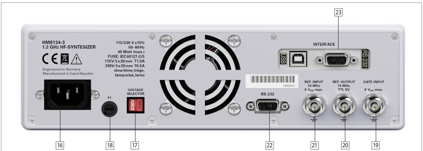
Fig. 2.2: Rear panel of the HM8134-3
